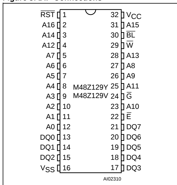
Figure 3. DIP Connections
