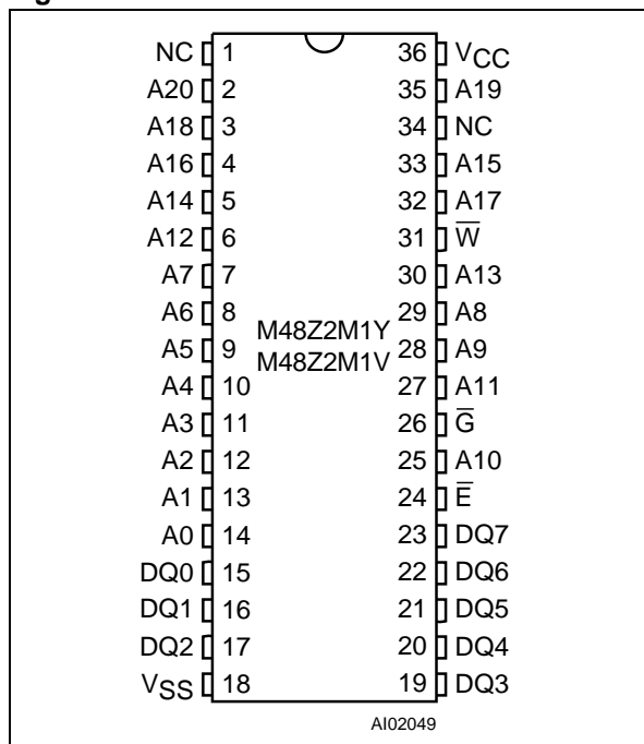
Figure 3. DIP Connections
