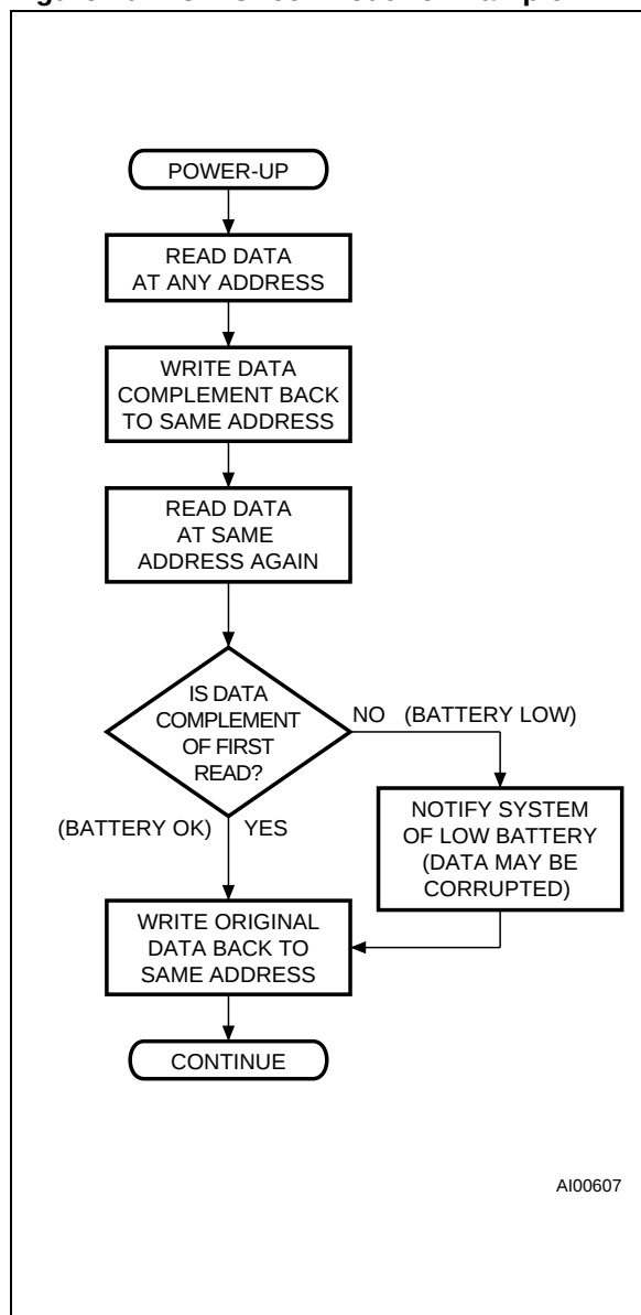
Figure 10. BOK Check Routine Example
