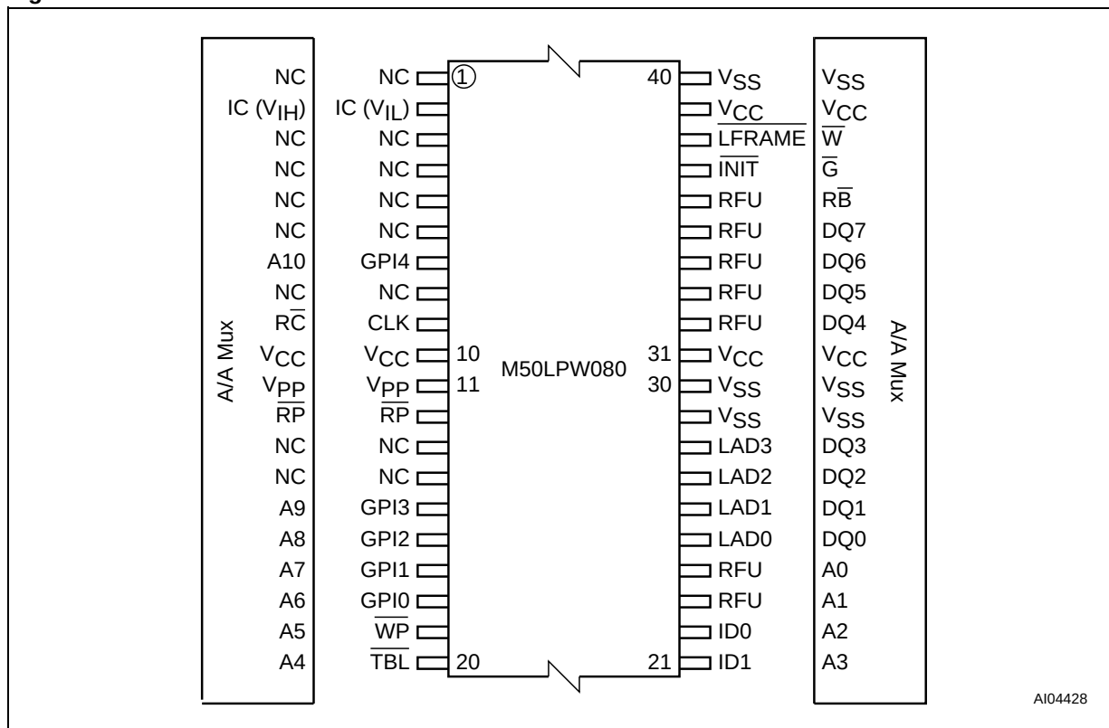
Figure 5. TSOP Connections
