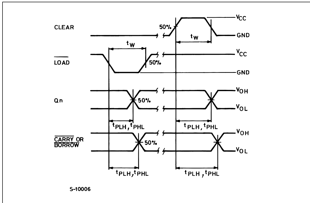
WAVEFORM 2 : PROPAGATION DELAY TIME, MINIMUM PULSE WIDTH (CLEAR, \overline{\text{LOAD}} ) ( f=1\text{MHz} ; 50% duty cycle)
