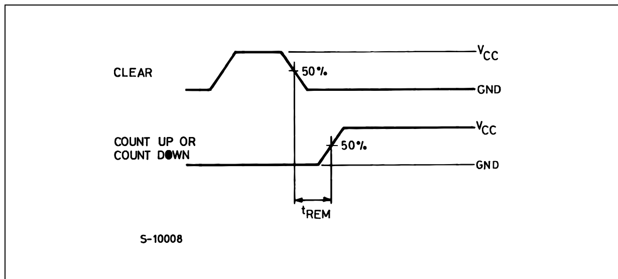
WAVEFORM 4: MINIMUM REMOVAL TIME (COUNT UP OR DOWN TO CLEAR) (f=1MHz; 50% duty cycle)
