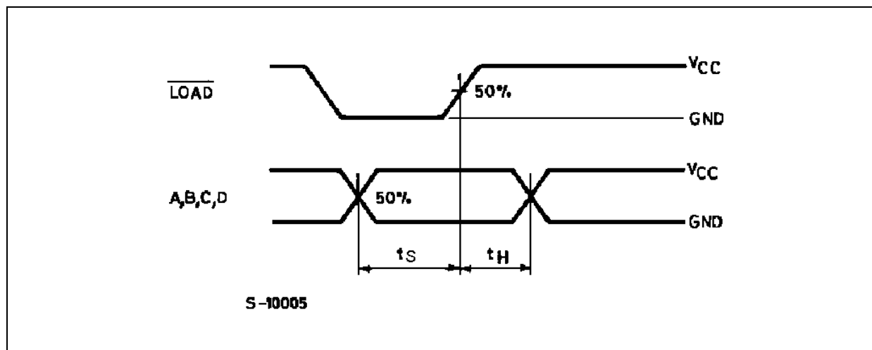
WAVEFORM 3 : SETUP AND HOLD TIME (A, B, C, D to \overline{\text{LOAD}} ) ( f=1\text{MHz} ; 50% duty cycle)
