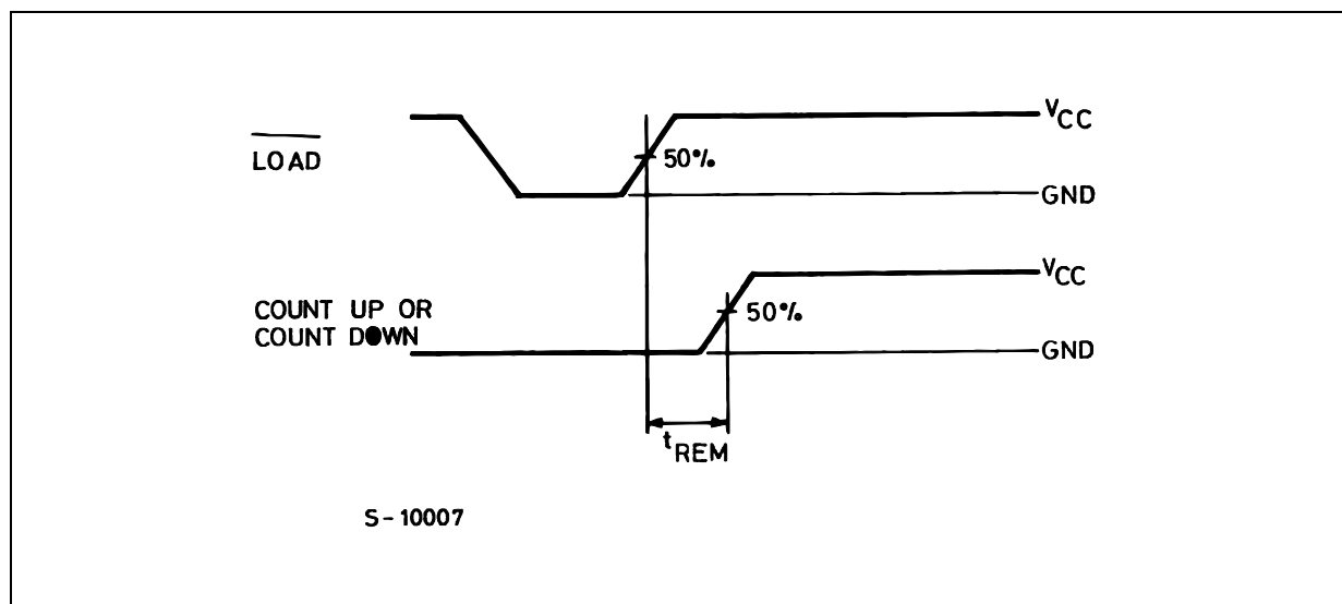
WAVEFORM 5 : MINIMUM REMOVAL TIME (COUNT UP OR DOWN TO \overline{LOAD} ) (f=1MHz; 50% duty cycle)
