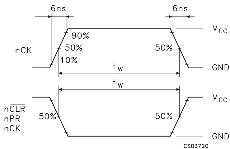
WAVEFORM 4 : MINIMUM PULSE WIDTH ( \overline{nCLR} , \overline{nPR} , nCK ) ( f=1\text{MHz} ; 50% duty cycle)
