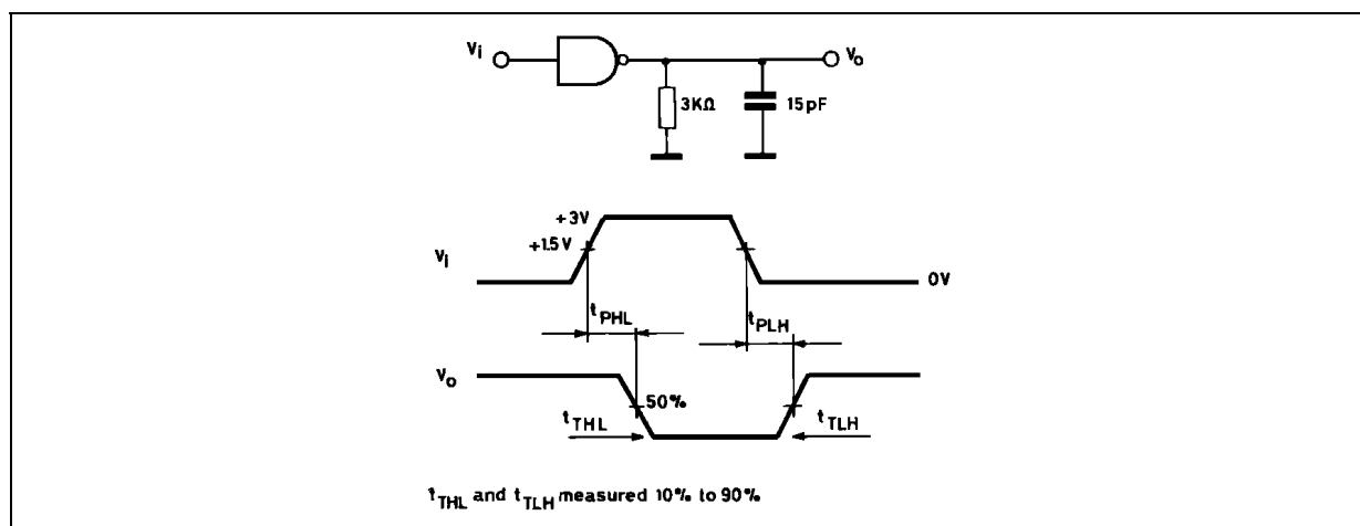
Figure 6 : Switching Response
