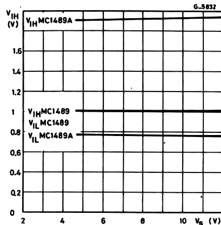
Figure 11 : Input Threshold versus Power Supply Voltag
