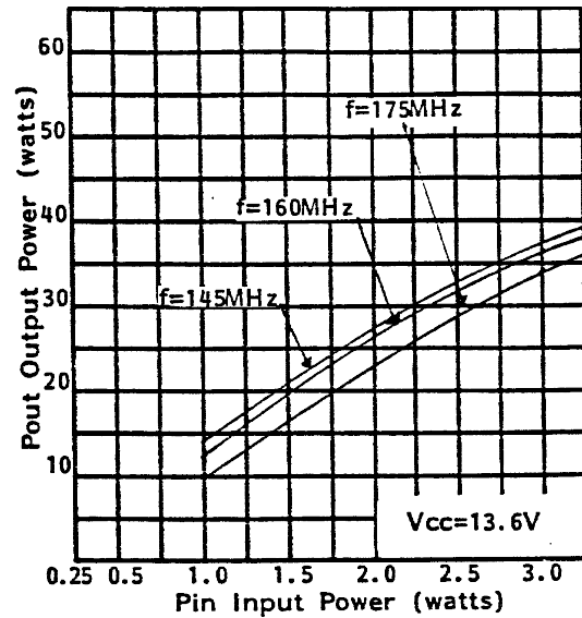
POWER OUTPUT vs POWER INPUT
