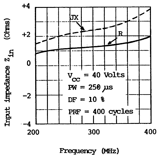
TYPICAL INPUT IMPEDANCE
