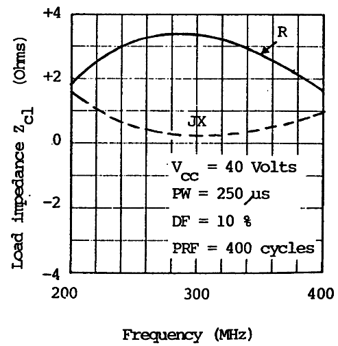
TYPICAL COLLECTOR LOAD IMPEDANCE
