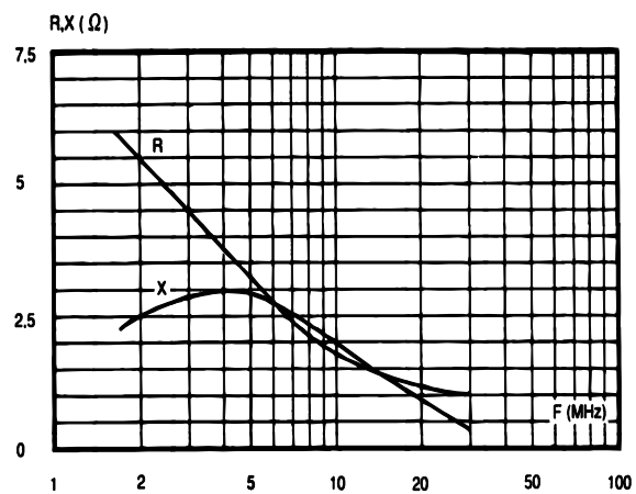
Figure 9. Typical Input Impedance
