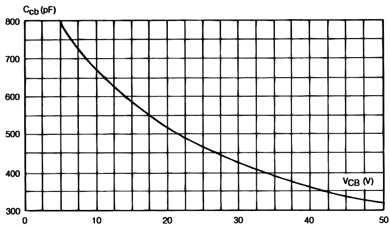
COLLECTOR BASE CAPACITANCE vs COLLECTOR EMITTER VOLTAGE
