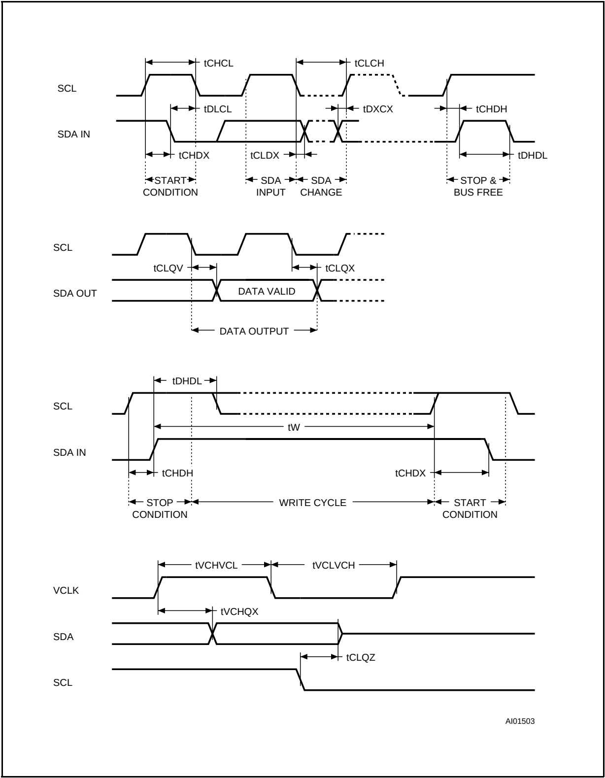
Figure 7. AC Waveforms
