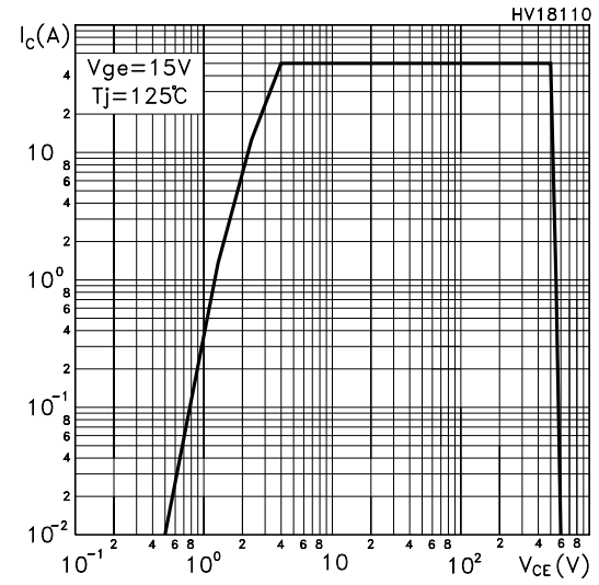
Turn-Off SOA
