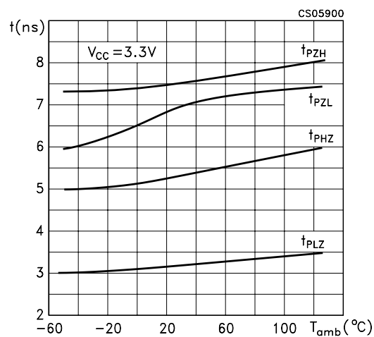
Figure 7 : Propagation Delay Enable to Output
