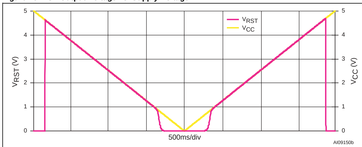
Figure 23. \overline{\text{RST}} Output Voltage vs. Supply Voltage
