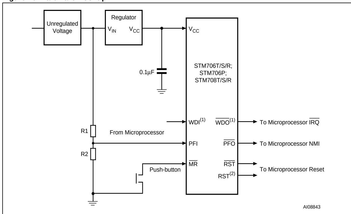
Figure 10. Hardware Hookup
