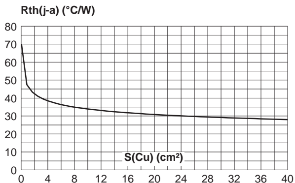
Fig. 8: Thermal resistance junction to ambient versus copper surface under tab (Epoxy printed circuit board FR4, copper thickness: 35µm)( D 2 PAK).
