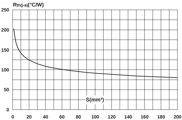
Fig. 9: Thermal resistance junction to ambient versus copper surface under tab (epoxy printed board FR4, Cu = 35μm, typical values).
