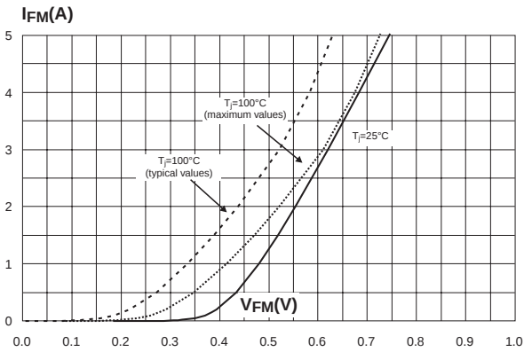
Fig. 7-2: Forward voltage drop versus forward current (low level, maximum values).
