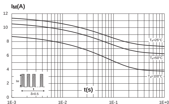
Fig. 3-1: Non repetitive surge peak forward current versus overload duration (maximum values) (DO-201AD, SMB).
