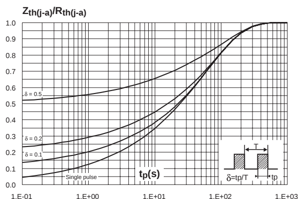
Fig. 4: Relative variation of thermal impedance junction to ambient versus pulse duration (DO-15).
