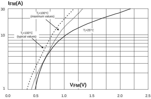
Fig. 7-1: Forward voltage drop versus forward current (high level, maximum values).
