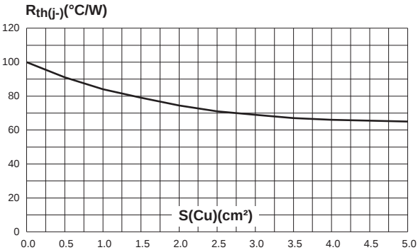
Fig. 8: Thermal resistance junction to ambient versus copper surface under each lead (Epoxy printed circuit board FR4, Cu: 35μm) (SMB).
