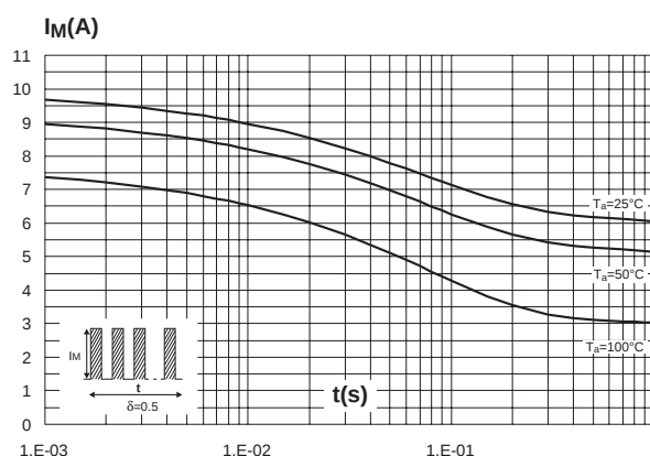
Fig. 3-2: Non repetitive surge peak forward current versus overload duration (maximum values) (DO-15).
