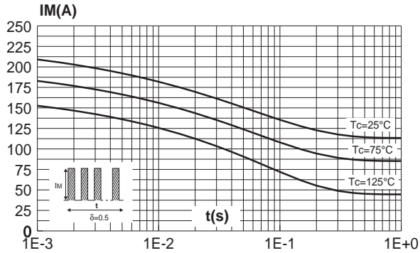
Fig. 3: Non repetitive surge peak forward current versus overload duration (maximum values, per
