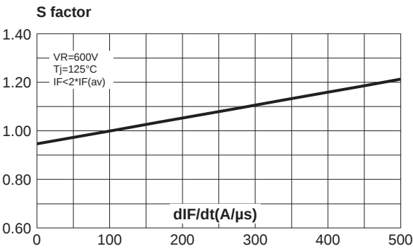
Fig. 7: Softness factor ( t_b/t_a ) versus dI_F/dt (typical values).
