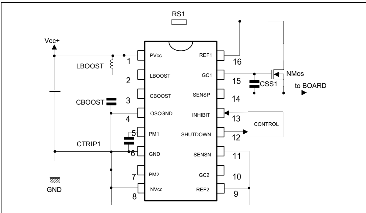
Figure 2 : SINGLE ELECTRONIC CIRCUIT BREAKER APPLICATION
