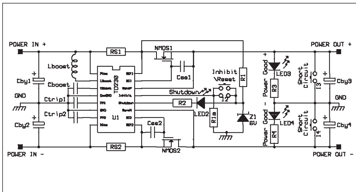
Figure 9C : Schematic
