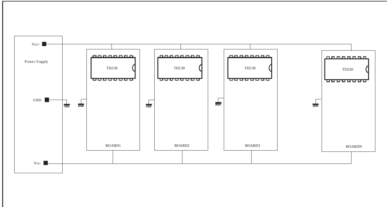
Figure 8 : Decentralized Protection
