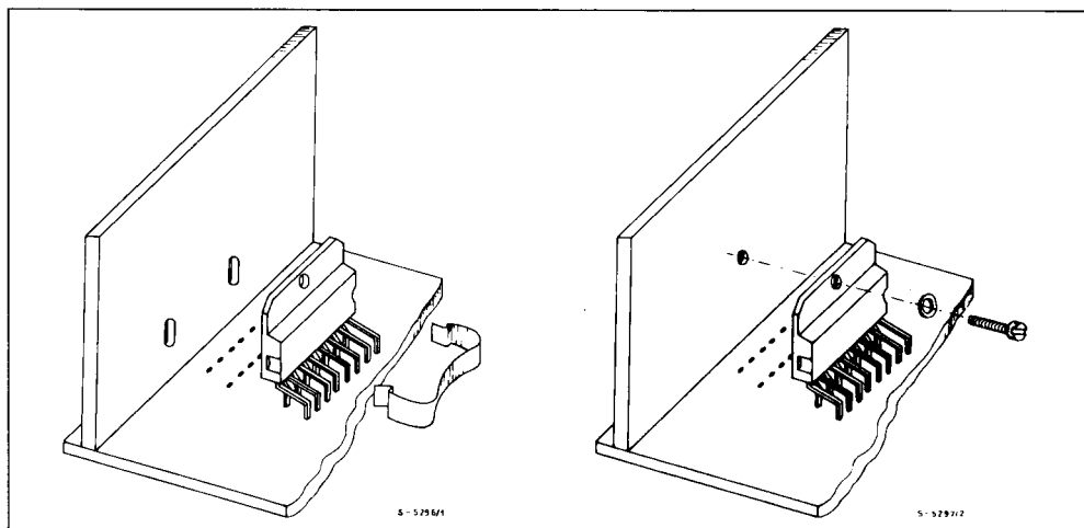
Figure 10 : Mounting Example.
