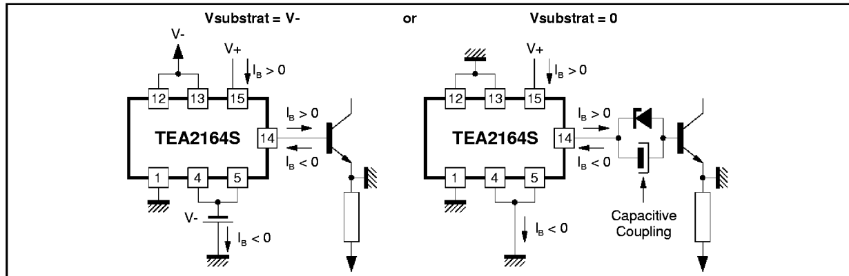
Figure 2 : Substrat Biasing
