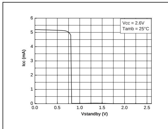
Fig. 75 : Current Consumption vs Standby Voltage @ V_{CC} = 2.6V
