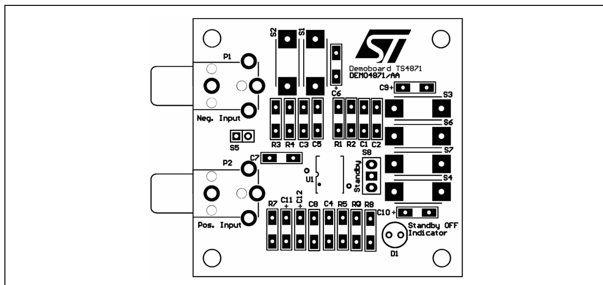
Fig. 82 : SO8 &amp; MiniSO8 Demoboard Components Side
