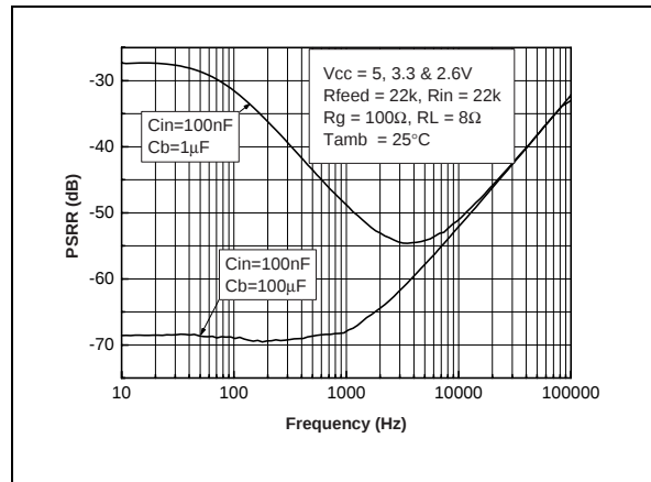
Fig. 85 : PSRR changes with C_b
