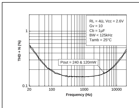
Fig. 64 : THD + N vs Frequency
