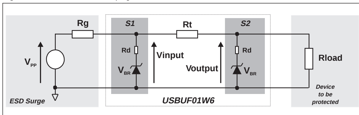
Fig. A5: USBUFFxxW6 ESD clamping behavior
