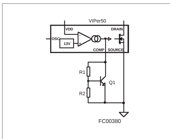
Figure 21: Current Limitation Circuit Example
