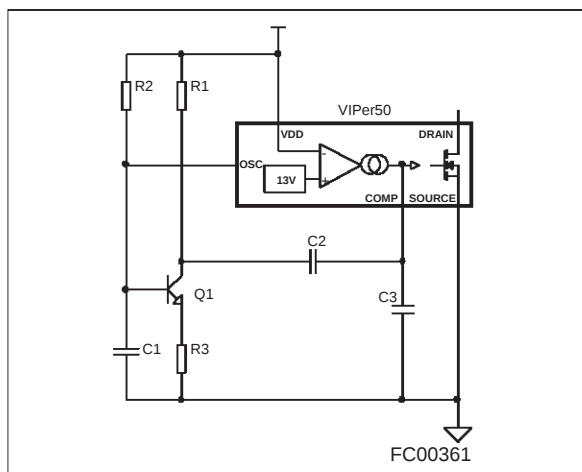
Figure 19: Slope Compensation
