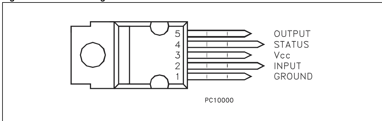
Figure 3. Connection Diagram
