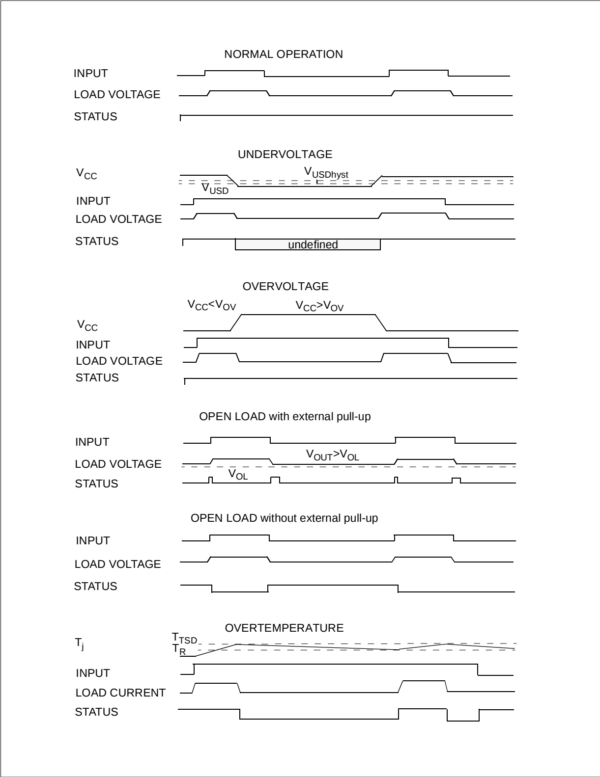
Figure 1: Waveforms
