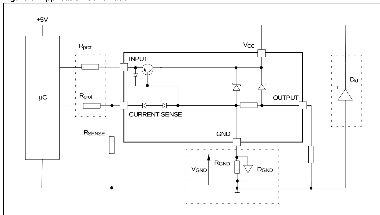
Figure 9. Application Schematic
