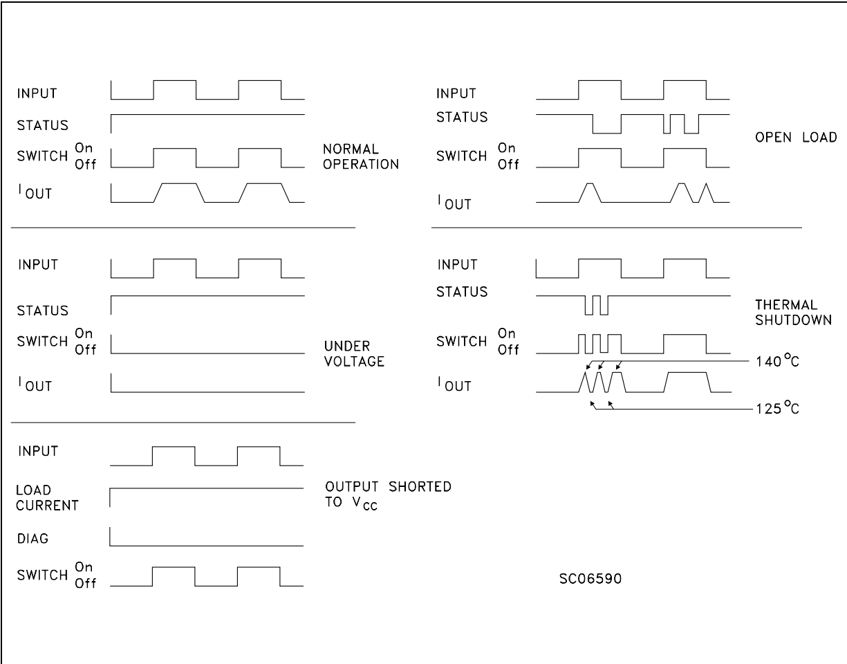
Figure 1: Waveforms
