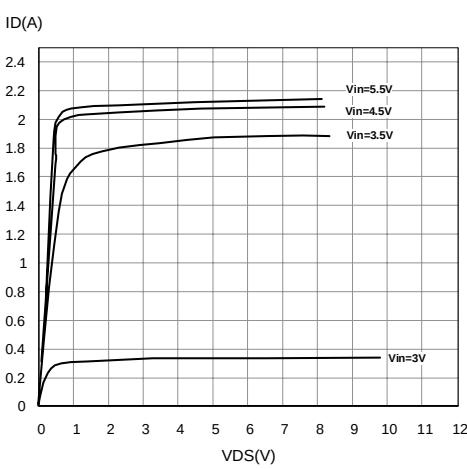
Output Characteristics
