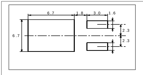
TAPE AND REEL SHIPMENT (suffix "13TR")
