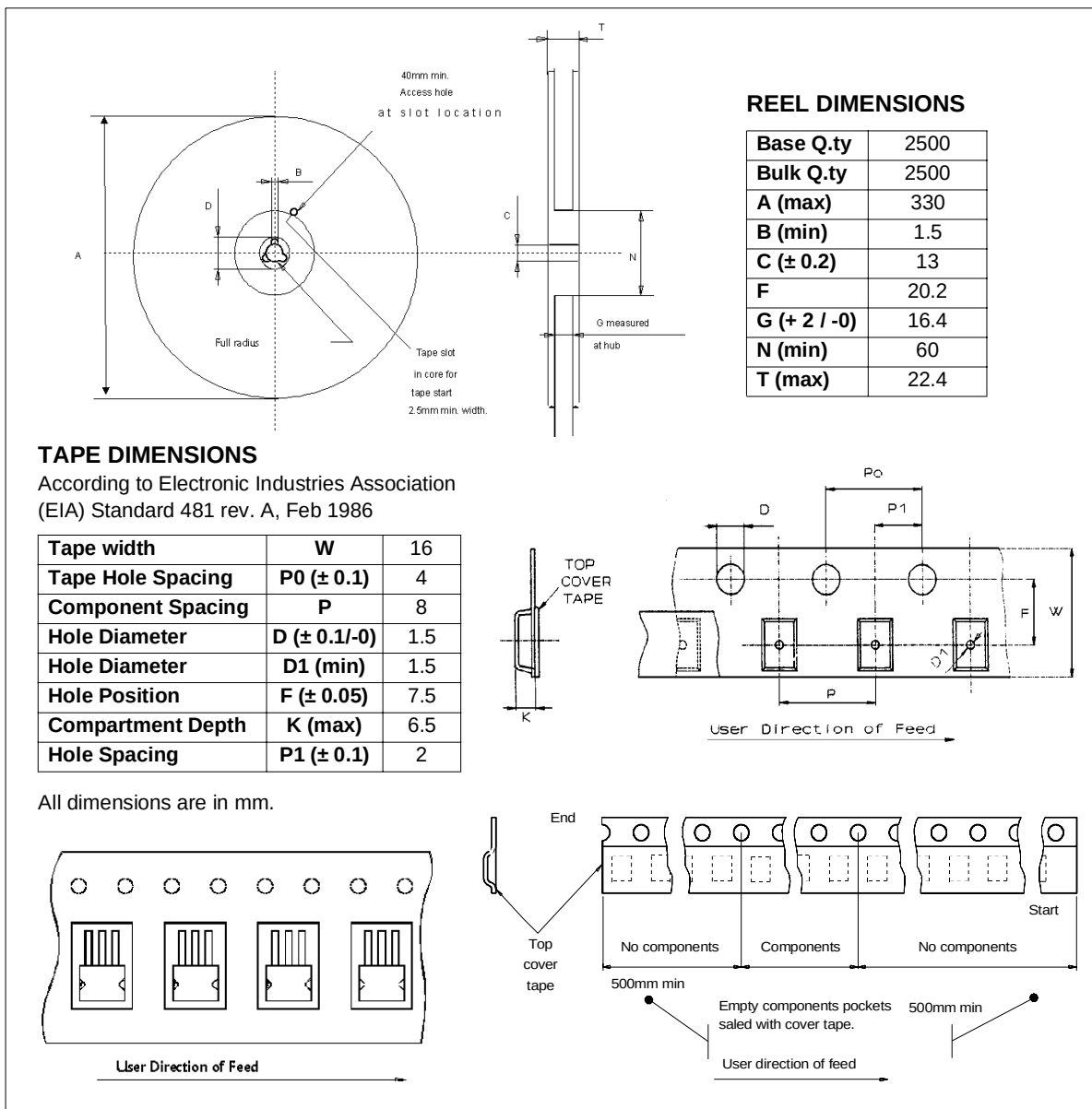
TAPE AND REEL SHIPMENT (suffix "13TR")
