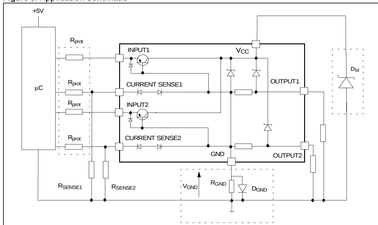
Figure 8. Application Schematic
