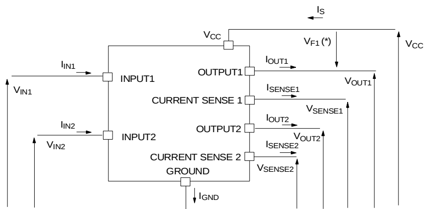
Figure 4. Current and Voltage Conventions
