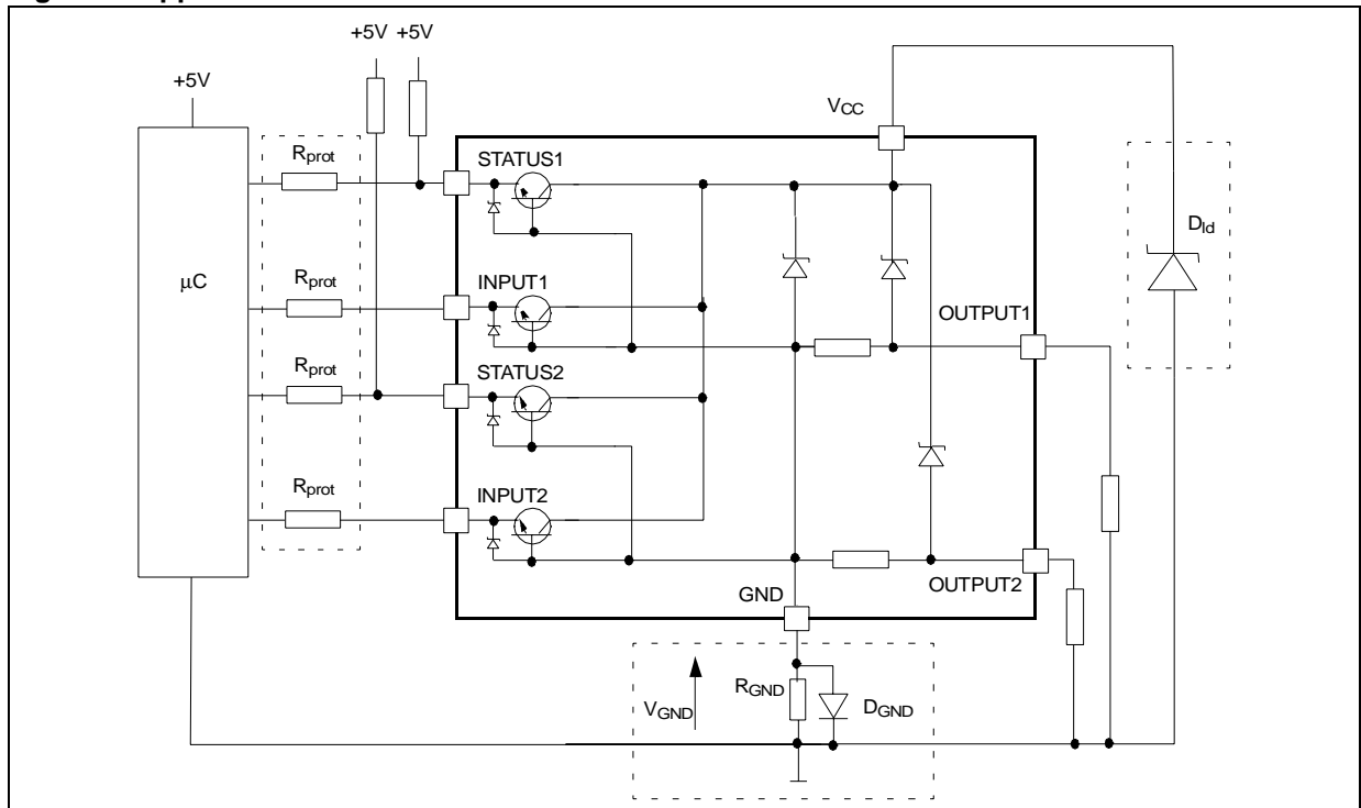
Figure 8. Application Schematic
