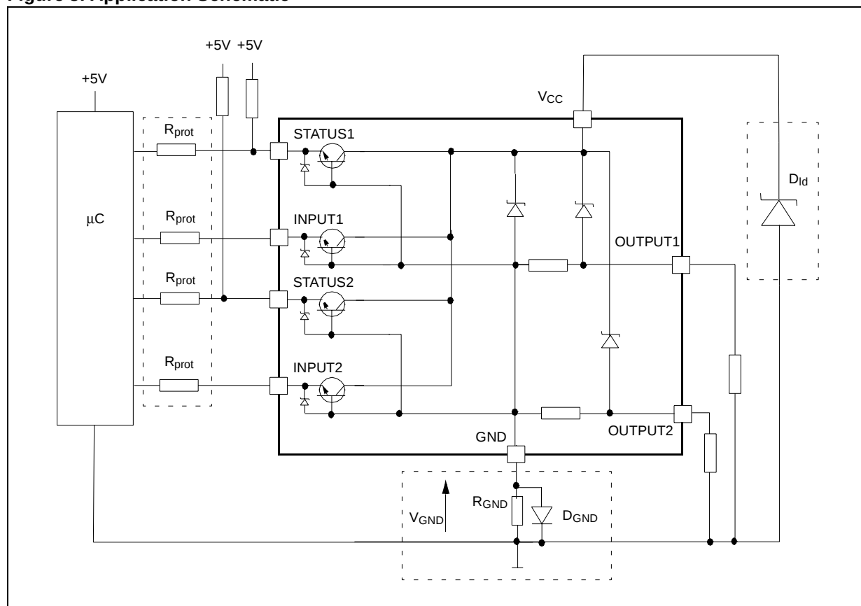
Figure 8. Application Schematic
