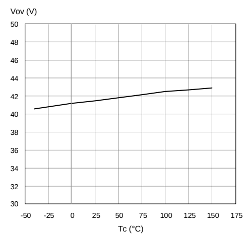
Figure 26. Overvoltage Shutdown
