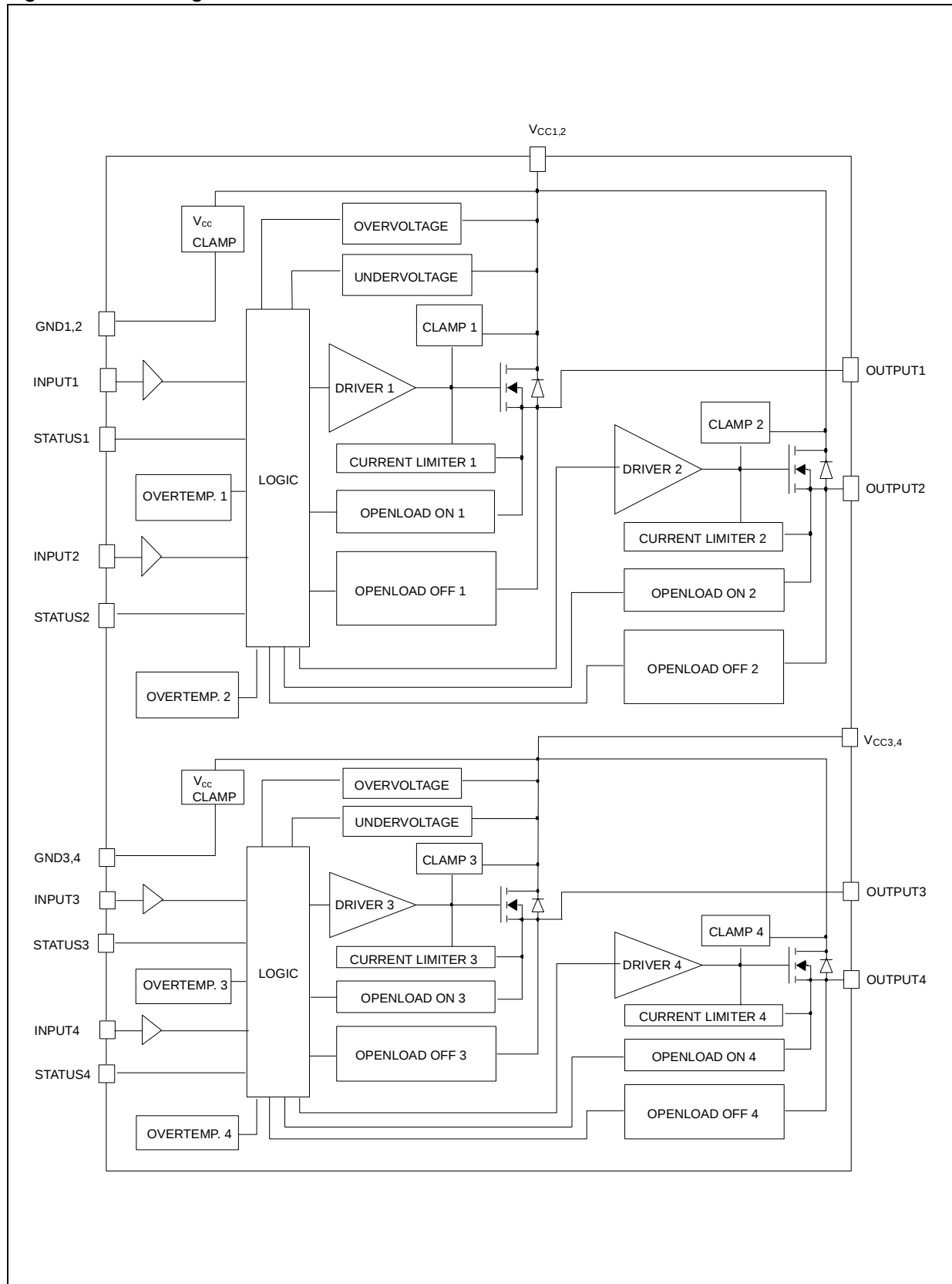
Figure 2. Block Diagram
