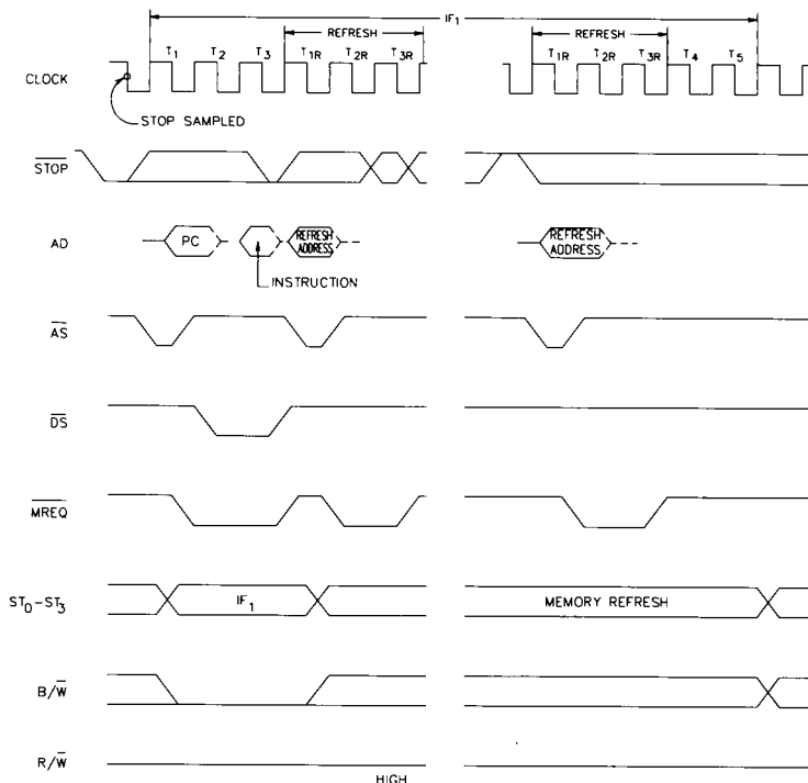
Figure 2-13. Stop Timing
