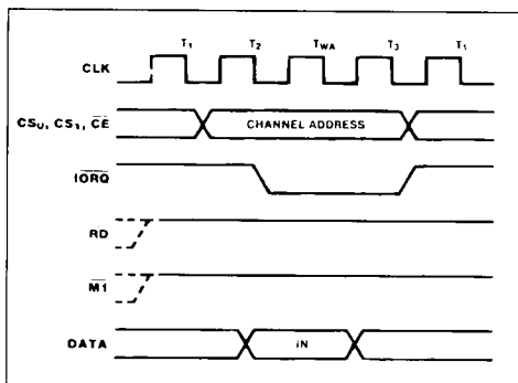
Figure 9 : Read Cycle Timing.
