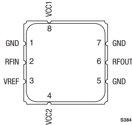
Figure 2. CX65100 Pinout– 8-Pin LCC Package (Top View)
