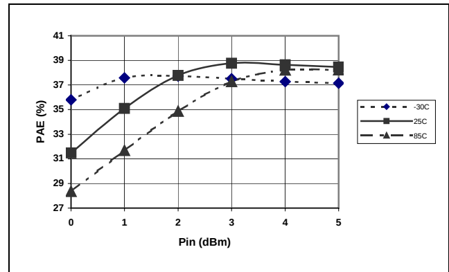
Figure 4. Typical PAE vs P_{IN} Over Temperature
