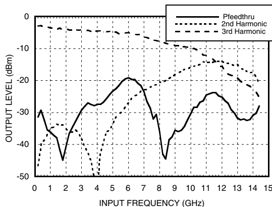
Output Harmonic
