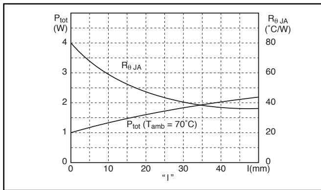
Figure 2 - Max. Power Dissipation And Junction To Ambient Thermal Resistance vs. Size "l" for 16 lead fused package.
