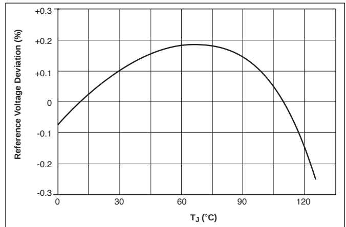
Bandgap Reference Voltage Deviation vs. Temperature
