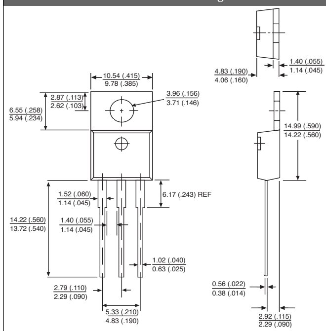
3 Lead TO-220 (T) Straight
