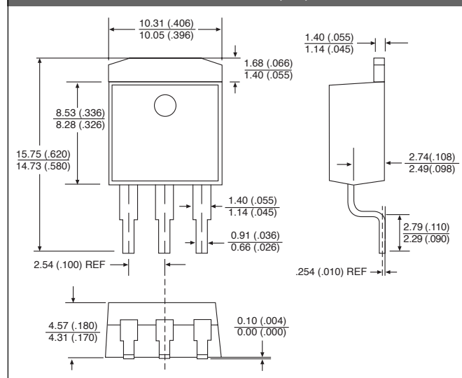
3 Lead D 2 PAK (DP)
