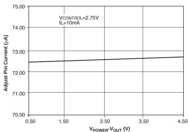
Adjust Pin Current vs V_{\text{POWER}} - V_{\text{OUT}}
