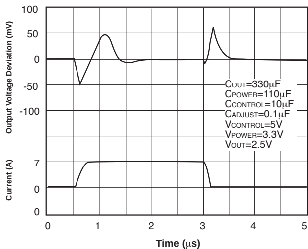
Transient Response
