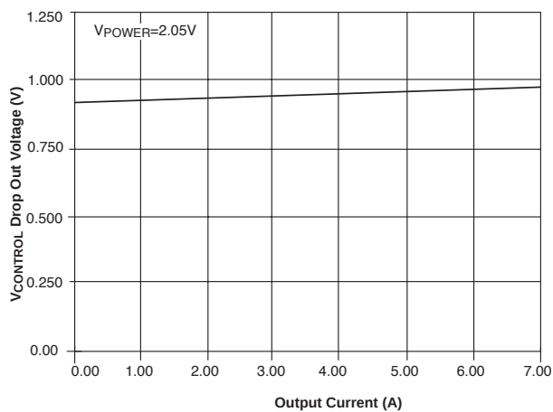
V_{\text{CONTROL}} Dropout Voltage vs I_{\text{OUT}}
