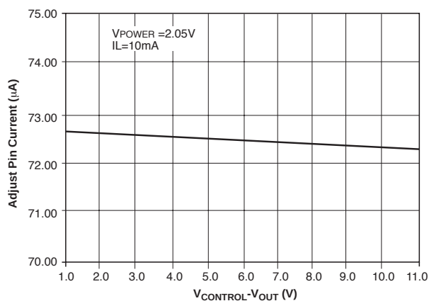
Adjust Pin Current vs V_{\text{CONTROL}} - V_{\text{OUT}}
