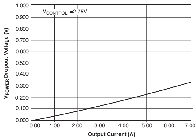
V_{\text{POWER}} Dropout Voltage vs I_{\text{OUT}}
