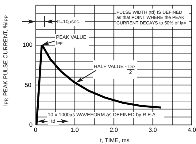
FIG. 3 - PULSE WAVEFORM
