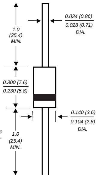
DO-204AC
