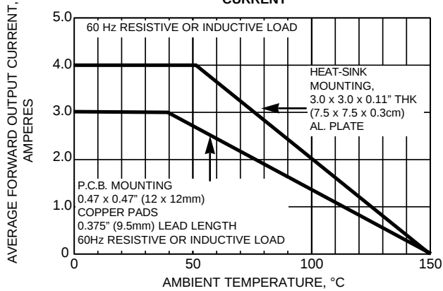
FIG. 1 - DERATING CURVES OUTPUT RECTIFIED CURRENT
